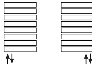
F ALLACCIAMENTO SCALDASALVIETTE MONOTUBO CLASSIC-AL BATH single pipe CLASSIC-AL BATH towel warmer connection
