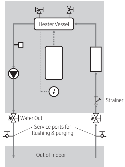
Hydro unit
